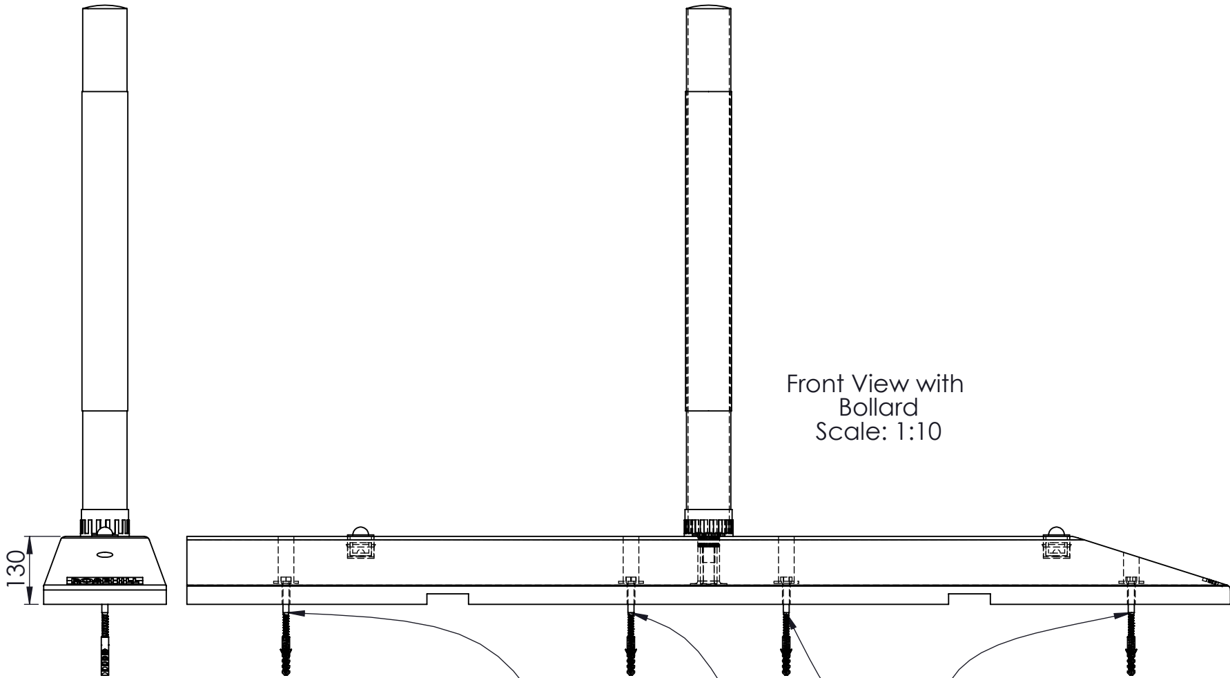
NCLD/1 - One Side Slope Weight : 57Kg
