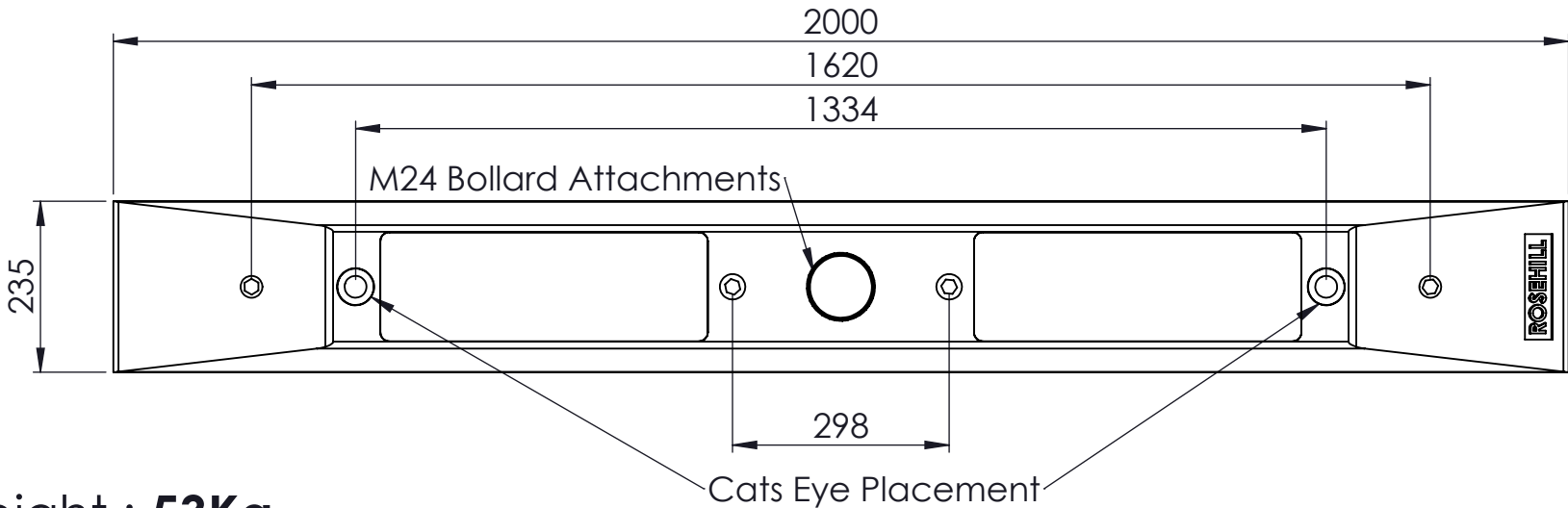
NCLD/2 - Two Slope Weight : 53Kg
