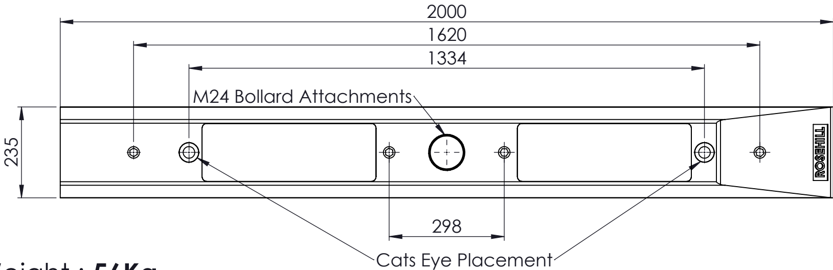
NCLD/1 - Single Slope Weight : 56Kg
