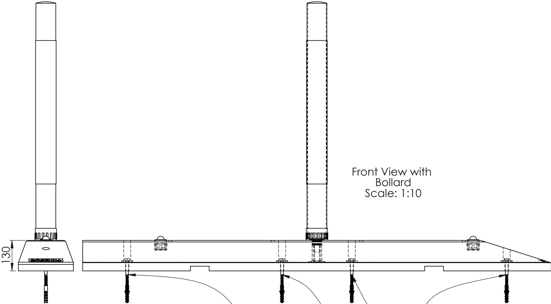
NCLD/1 - Single Slope Weight : 56Kg
