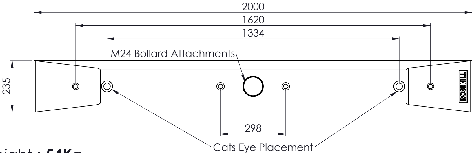
NCLD/2 - Two Slope Weight : 54Kg
