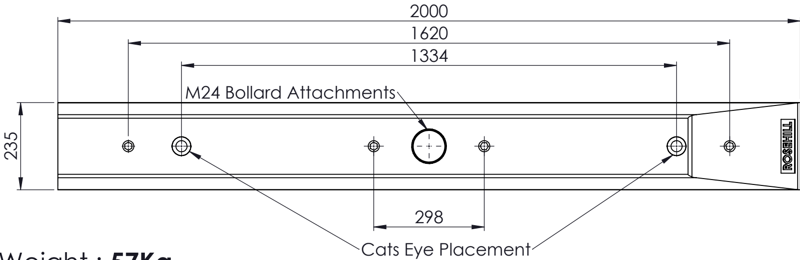
NCLD/1 - One Side Slope Weight : 57Kg
